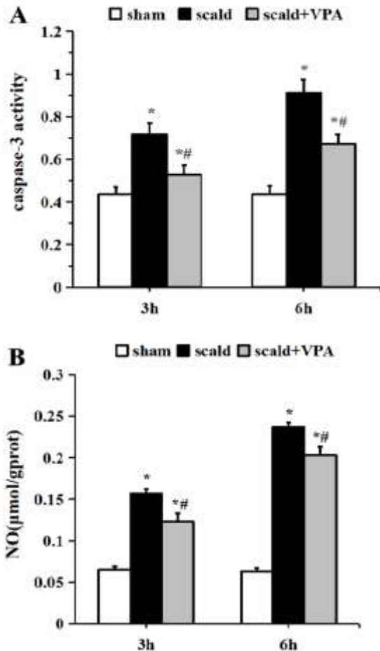
Fig. 3: Effect of VPA on caspase-3 activity and NO content in myocardial tissue. Caspase-3 activity(A) and NO content(B) were measured at 3 and 6 hours after scald, the values were expressed as the mean (SD), n = 8. * P < 0.05 , compared with the sham group; # P < 0.05 , compared with the scald group.
