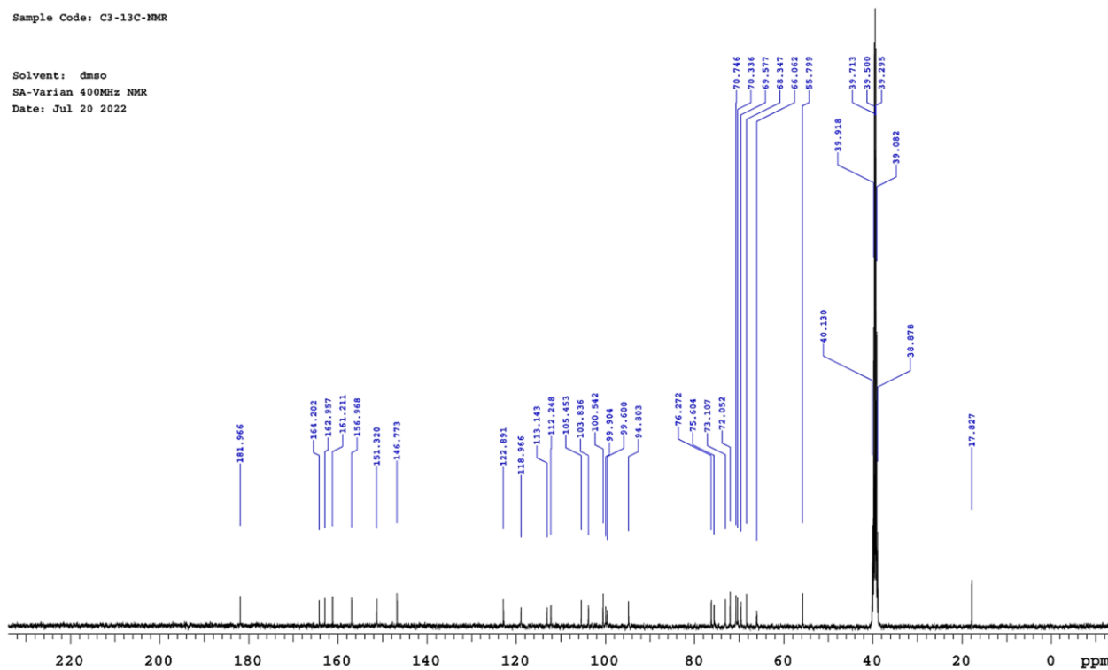
Fig. 7: Resultsof 13 C-NMR
