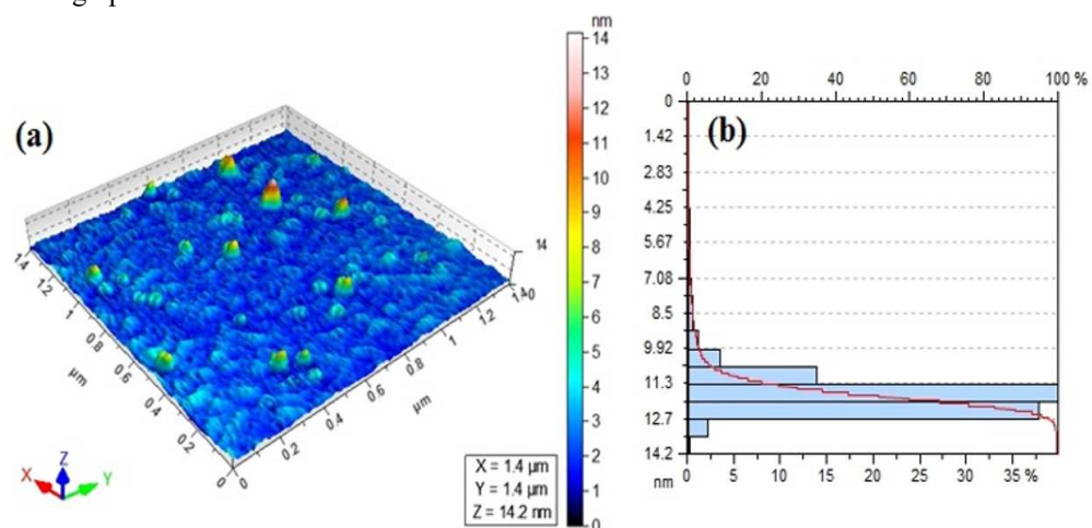
Fig. 6: AFM image of azithromycin coated silver nano-particles (Ag-AZM) (a) 3-D height image and (b) average particle height distribution graph.
