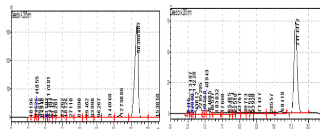
Fig. 5(a): HPLC peak of heated vitamin E & OA; (b): HPLC peak of F6
