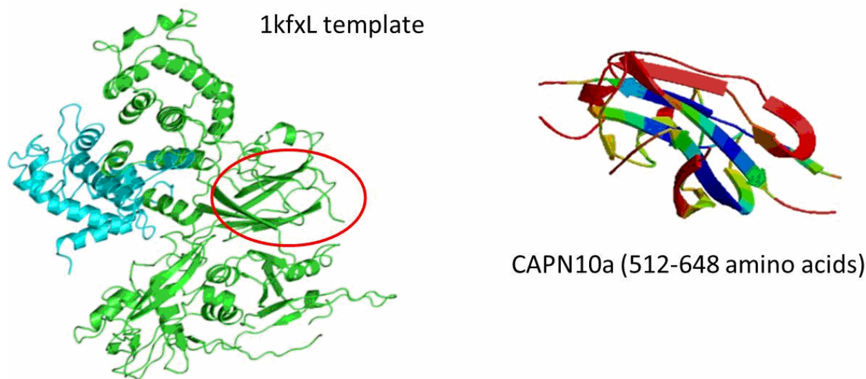
Fig. 5: 3D Structure of Calpain 10 (CAPN10) isoform a : created from Swiss model-ExPASy ( http://swissmodel.expasy.org ). PDB template 1kfxL hybridized 27% with CAPN10a. Estimated per-residue inaccuracy visualized using a color gradient from blue (more reliable regions) to red (potentially unreliable).
