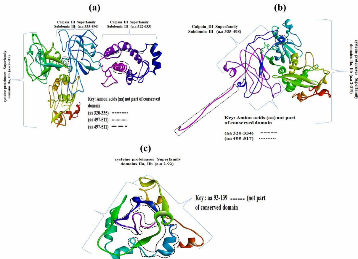
Fig. 2: 3D model of Calpain 10 a, c and g showing conserved domains. 3D Model was obtained using I-TASSER and Conserved regions determined using CDART and were identified on the model using Discovery Studio software.
