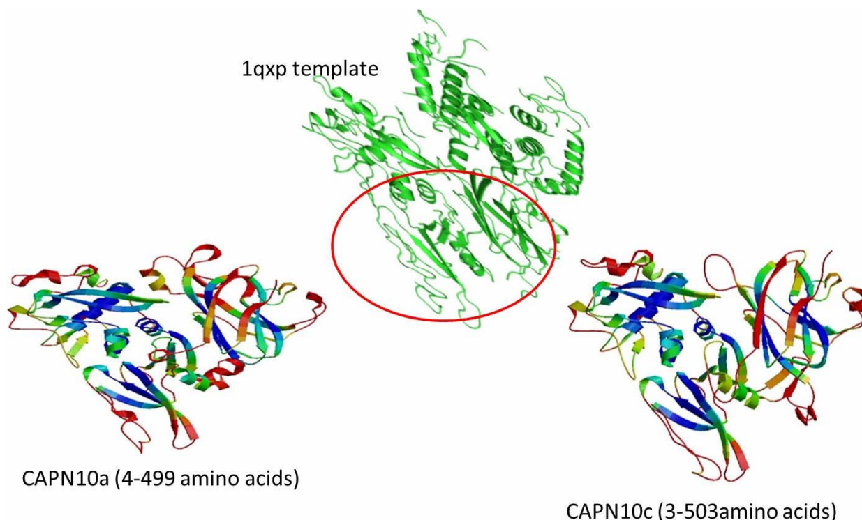
Fig. 4: 3D Structure of Calpain 10 (CAPN10) isoform a & c : created from Swiss model-ExPASy ( http://swissmodel.expasy.org ). PDB template 1qxp hybridized 29% and 28.2% with CAPN10 a and c respectively. Estimated per-residue inaccuracy visualized using a color gradient from blue (more reliable regions) to red (potentially unreliable).
