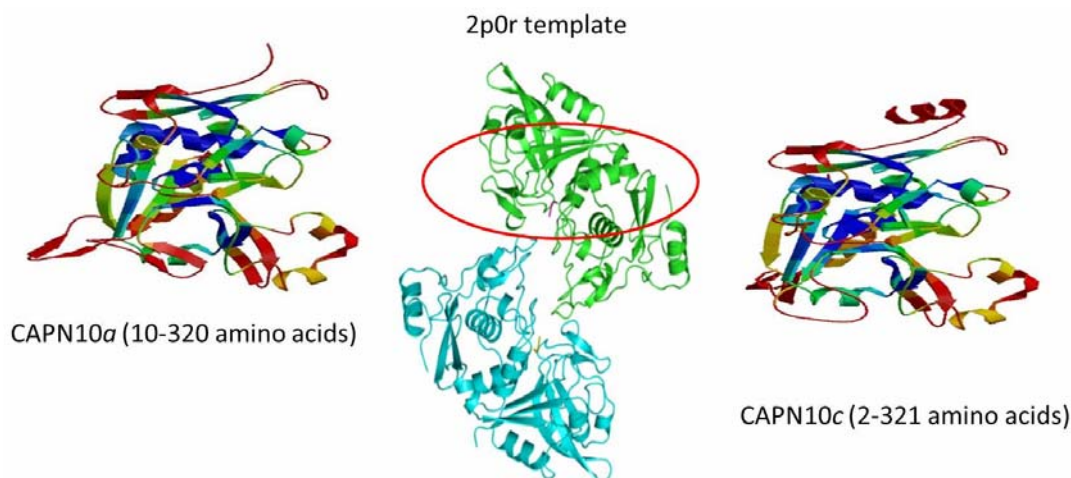
Fig. 3: 3D Structure of Calpain 10 (CAPN10) isoform a & c ; created from Swiss model-ExPASy ( http://swissmodel.expasy.org ). PDB template 2p0r hybridized 32% and 31.8% with CAPN10 a and c respectively. Estimated per-residue inaccuracy visualized using a color gradient from blue (more reliable regions) to red (potentially unreliable).
