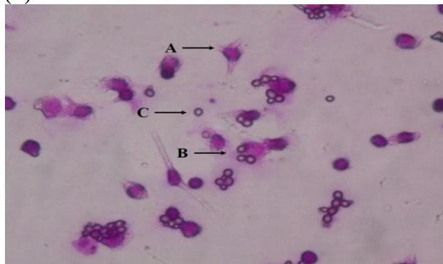
Fig. 10: Phagocytic activity of macrophages against Candida albicans . Control cells (CC) and different levels concentration of DMSO (DMSO), Massoia Oil (MO), Massoia Nanoemulsion (MN) and MN Base (B).
