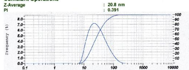
Fig. 2: PSA result for massoia oil nanoemulsion particle size.
