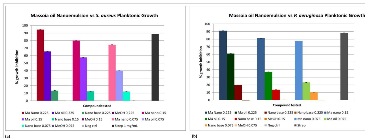
Fig. 5: Massoia oil nanoemulsion antibacterial activity against Pseudomonas aeruginosa and Staphylococcus aureus .
