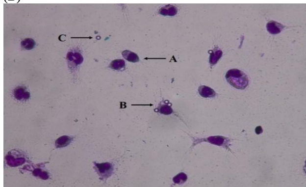
Fig. 8: Macrophages were observed under a light microscope magnification 10x40 times, non-specific
