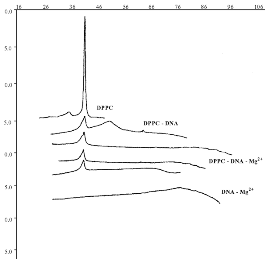
Fig. DSC heating scans of the main phase transition of DPPC multilayers and unilamellar vesicles obtained from them, upon their associations with various amounts of calf thymus DNA and 0.5 mM Mg 2+ . Each complex is denoted in the abbreviated form. Data is presented as excess apparent heat capacity vs. temperature curves. Details of sample preparation and measurements are outlined in Materials and Methods.
